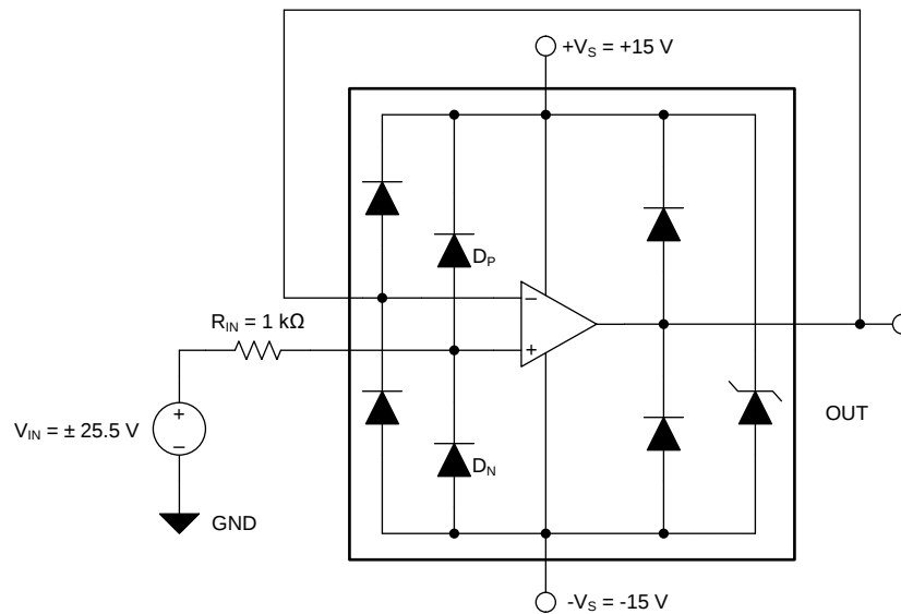
Figure 2. Limiting the Input Current
