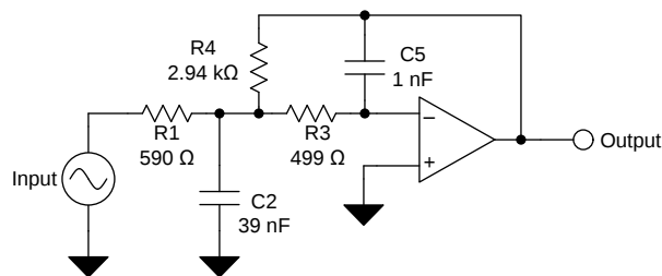
Figure 7. Typical OPA828 Application Schematic
