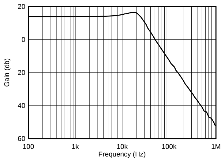
Figure 8. Low-Pass Filter Transfer Function
