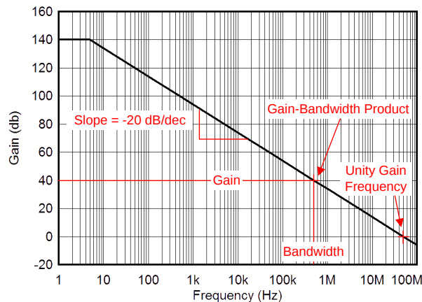
Figure 6. Gain-Bandwidth Product and Unity Gain Frequency
