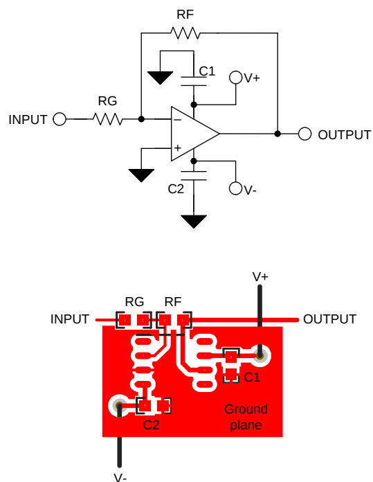
Figure 9. OPA828 PCB Example
