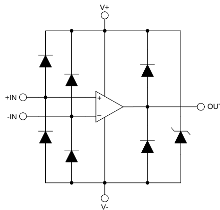
Figure 1. Equivalent Internal ESD Circuitry
