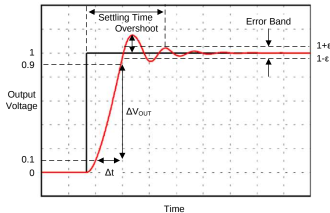
Figure 5. Settling Time
