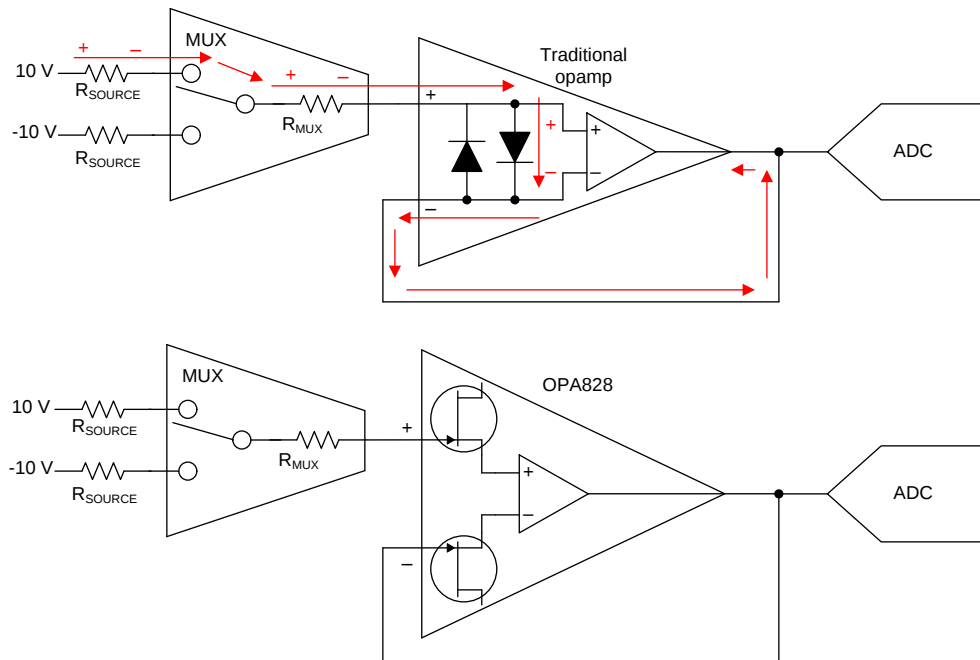
Figure 4. Typical Multiplexed System Block Diagram
