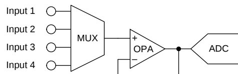
Figure 3. Typical Multiplexed System Block Diagram
