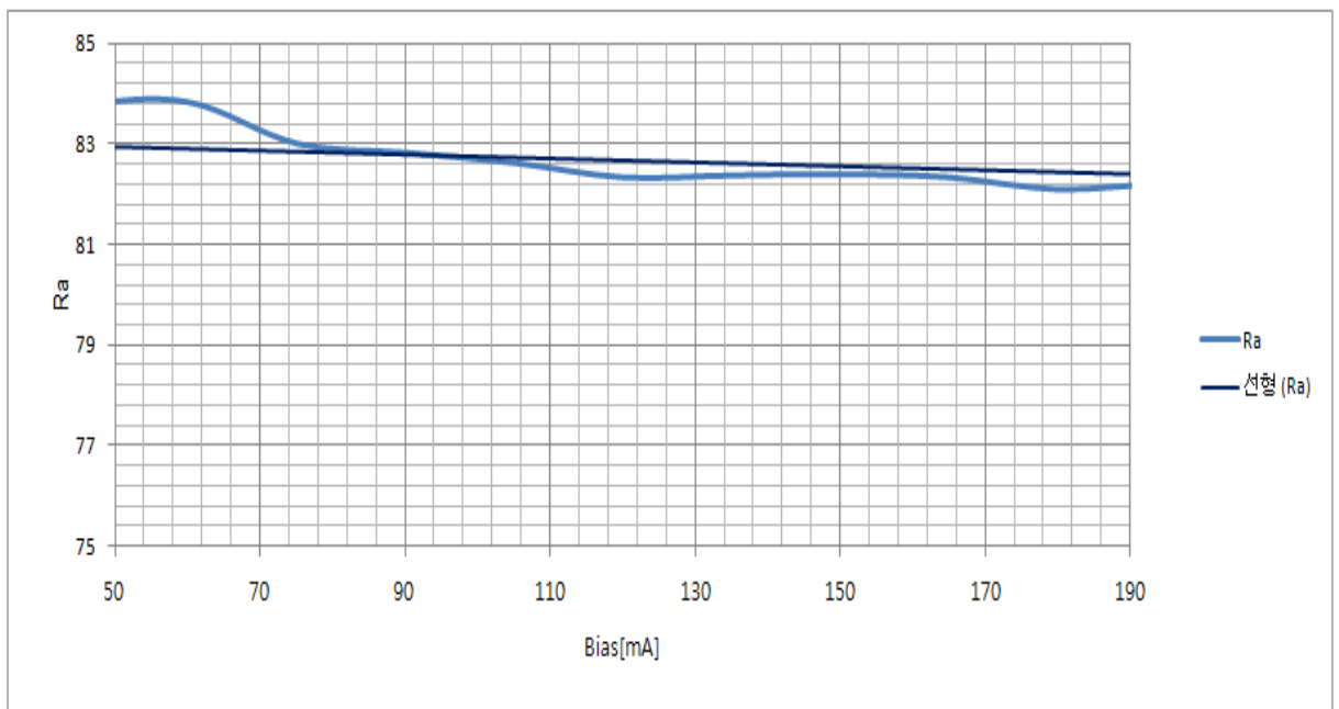
Fig.6 Forward current vs Color Rendering Index
