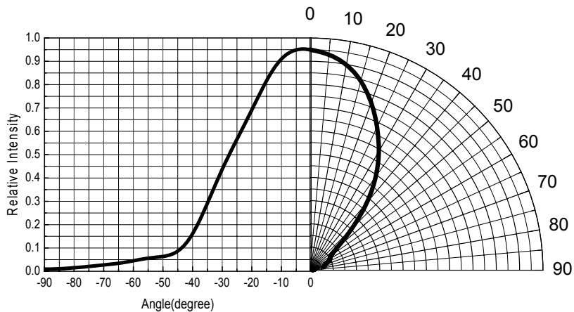
Relative Radiant Intensity vs. Angular Displacement
