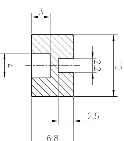
SECTION B-B' (2:1)
