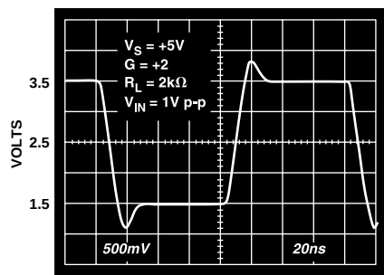
Figure 32. Large Signal Step Response; V_S = +5 V , G = +2
