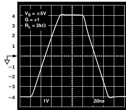
Figure 35. Large Signal Step Response; V_S = \pm 5 V , G = +1
