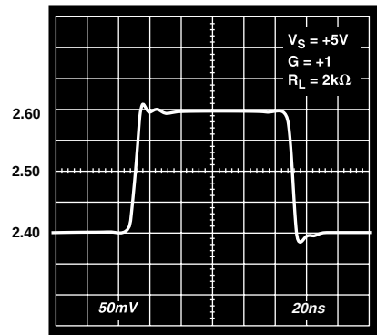
Figure 31. AD8051/AD8052 200 mV Step Response; V_S = +5 V , G = +1
