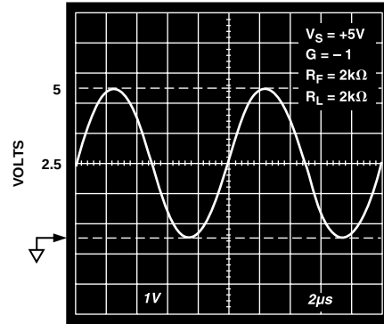
Figure 33. Output Swing; G = -1 , R_L = +2 k\Omega
