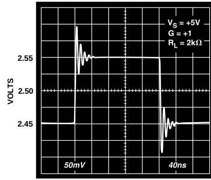
Figure 34. AD8054 100 mV Step Response; V_S = +5 V , G = +1
